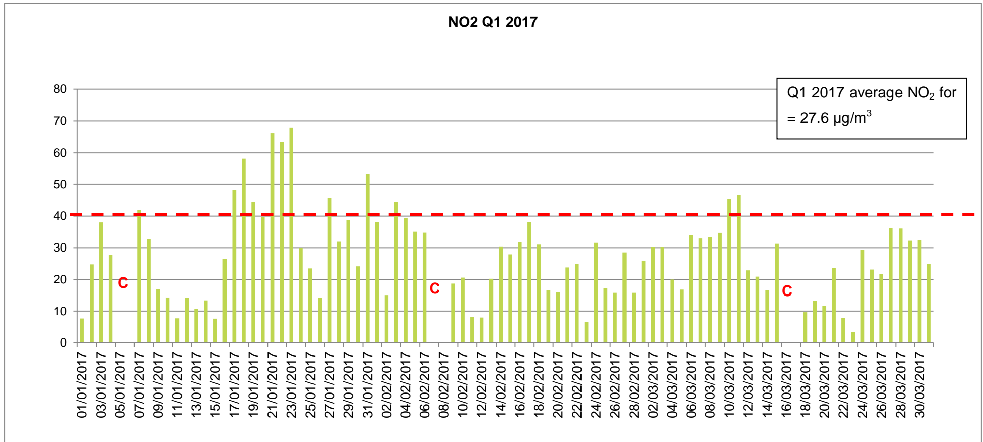
Figure 4 Daily Average NO 2 Q1 2017
