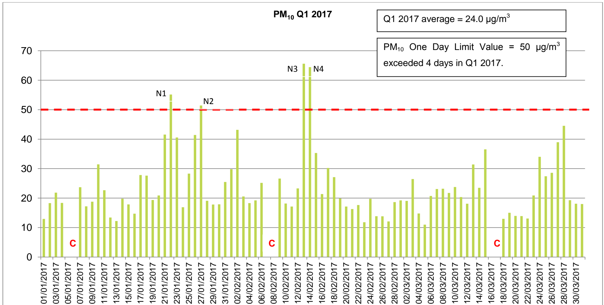
Figure 5 Daily Average PM 10 Q1 2017
