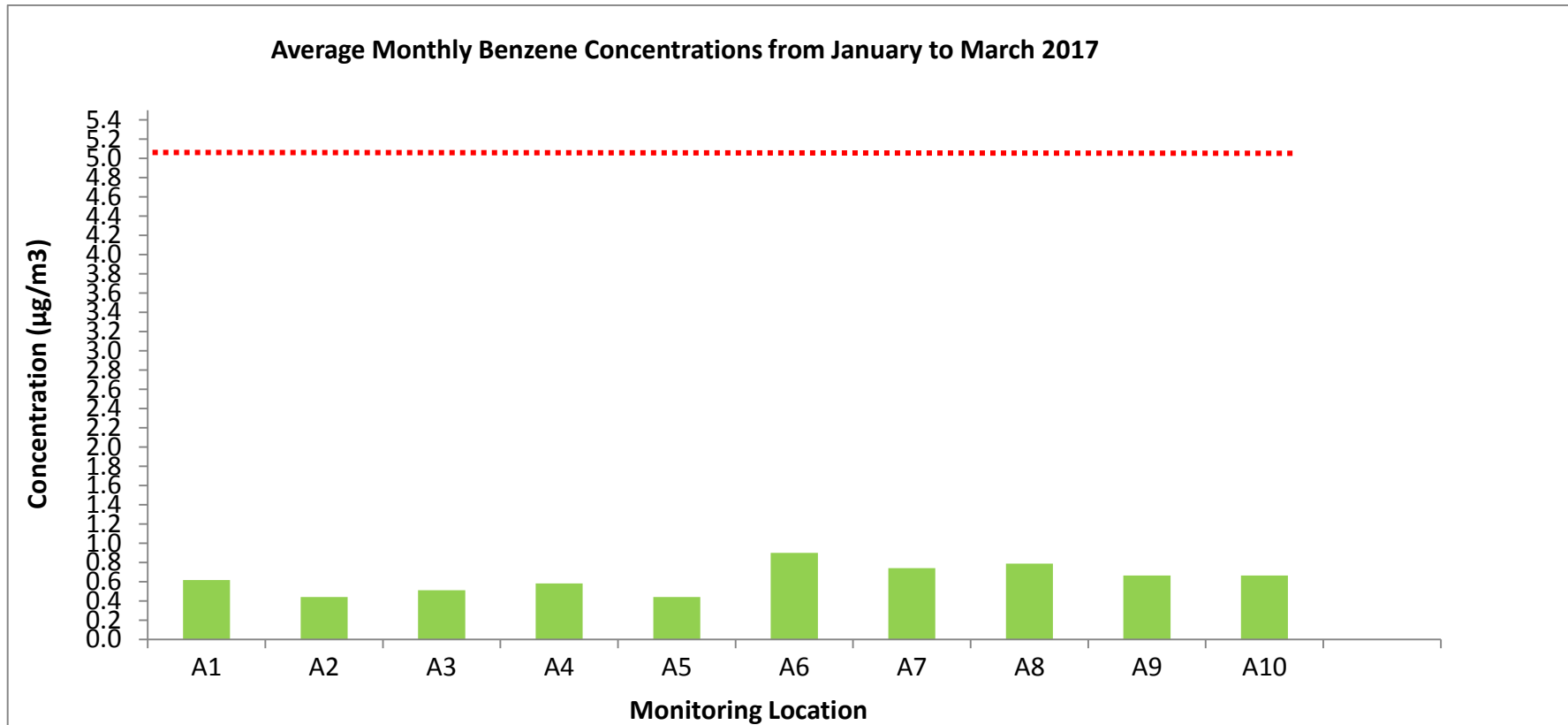
Figure 3 Average Monthly Benzene (C 6 H 6 ) Concentrations Q1 2017
