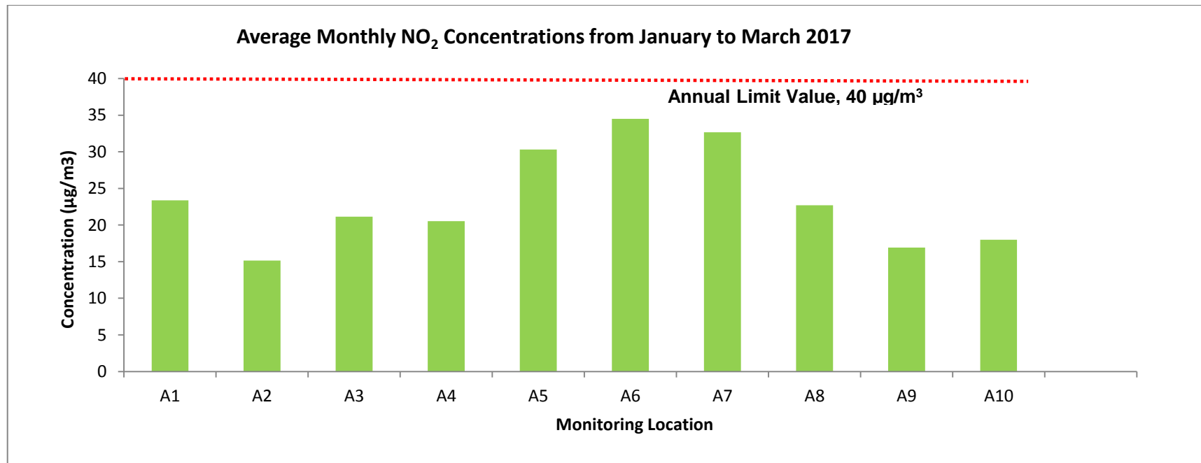
Figure 2 Average Monthly NO 2 Concentrations Q1 2017
